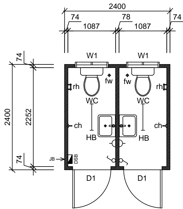
2.4x2.4m Toilet Block - Floor Plan
