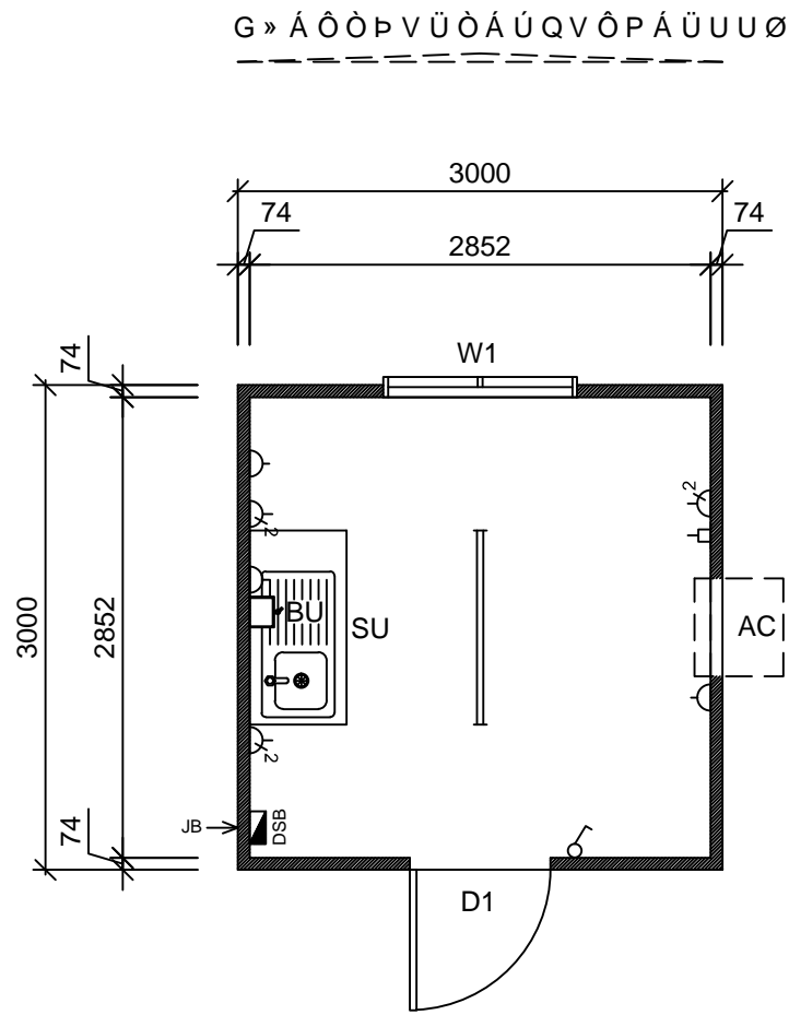
3.0x3.0m Crib Room - Floor Plan Scale 1:50
