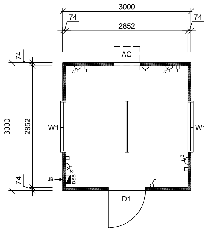
3.0x3.0m Office - Floor Plan
