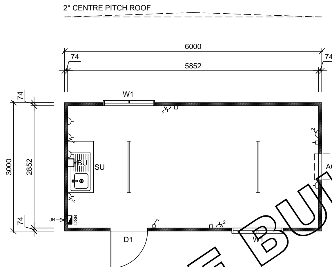
6.0x3.0m Crib Room - Floor Plan
