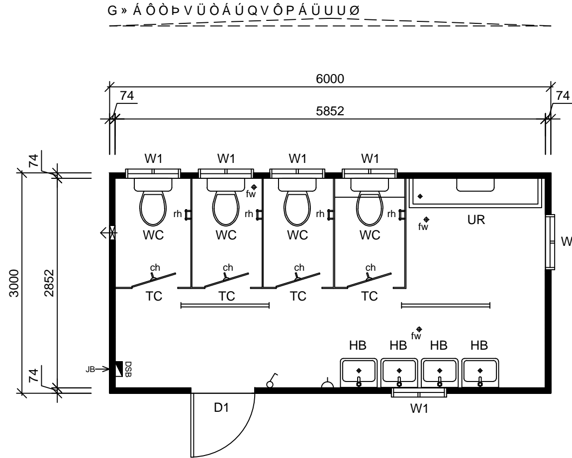
6.0x3.0m Male Toilet Block - Floor Plan
