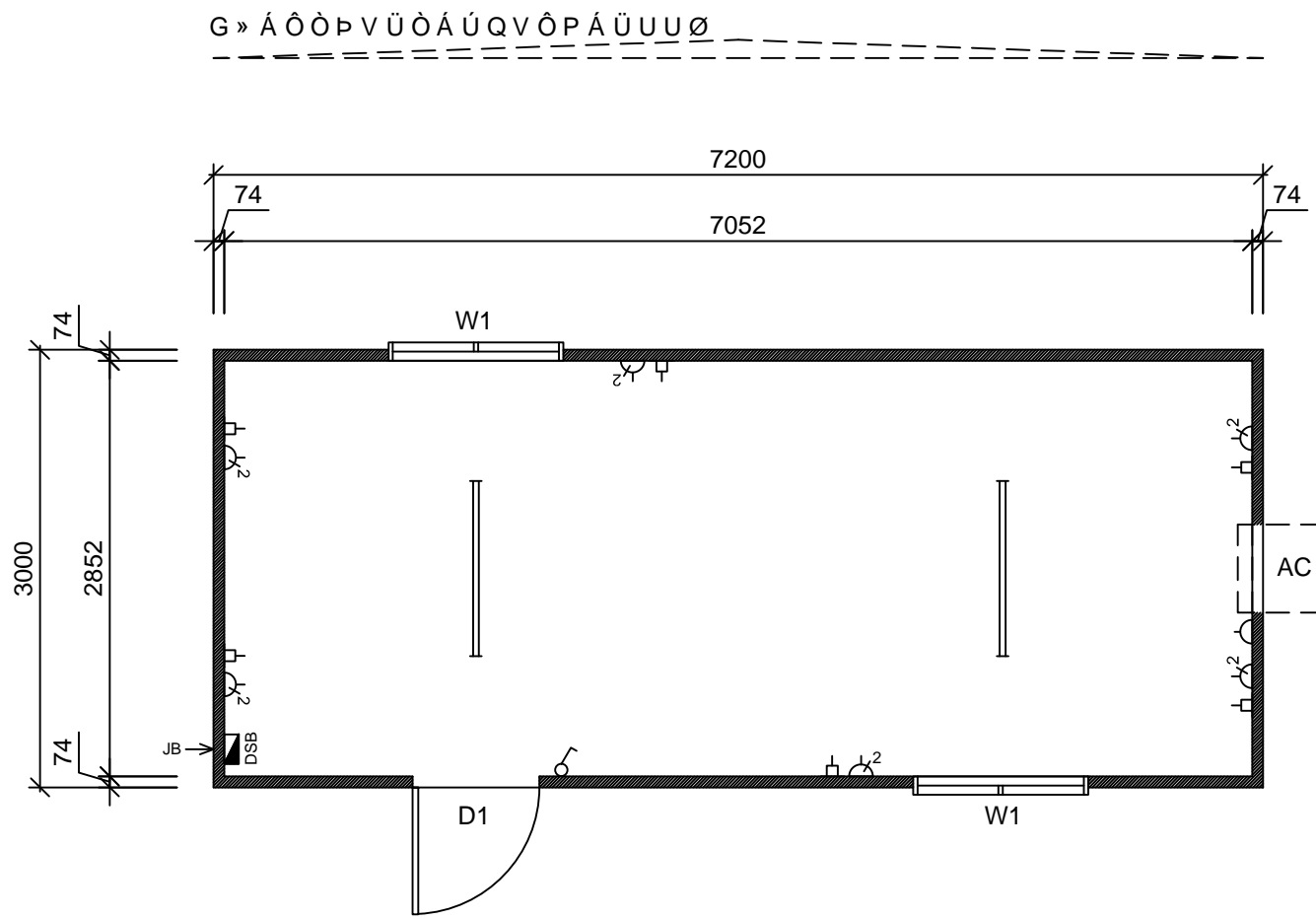
7.2x3.0m Office - Floor Plan
