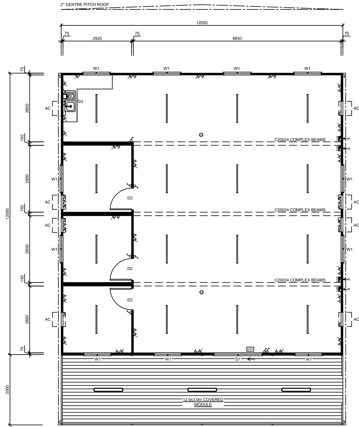
12.0x12.0m Complex & 12.0x3.0m Covered Deck - Floor Plan
